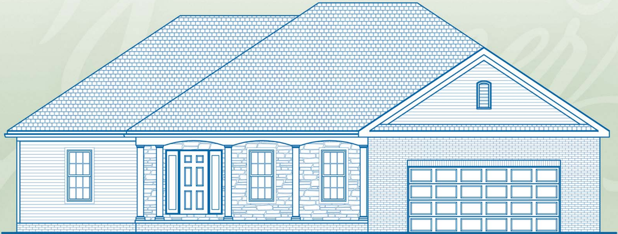
"MY KIND OF TOWN" 3 BEDROOM - RANCH FRONT ELEVATION "B" 2,182 SQUARE FEET
